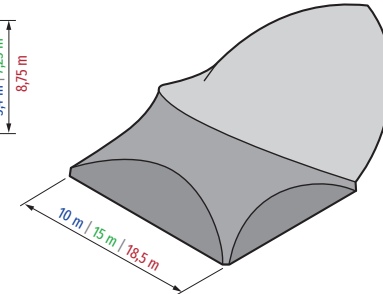
CLOSED ON ONE END – CLOSED ARCHES Covered area 130 m 2 | 285 m 2 | 423 m 2
